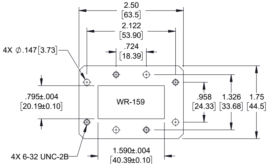
FLANGE DETAIL
