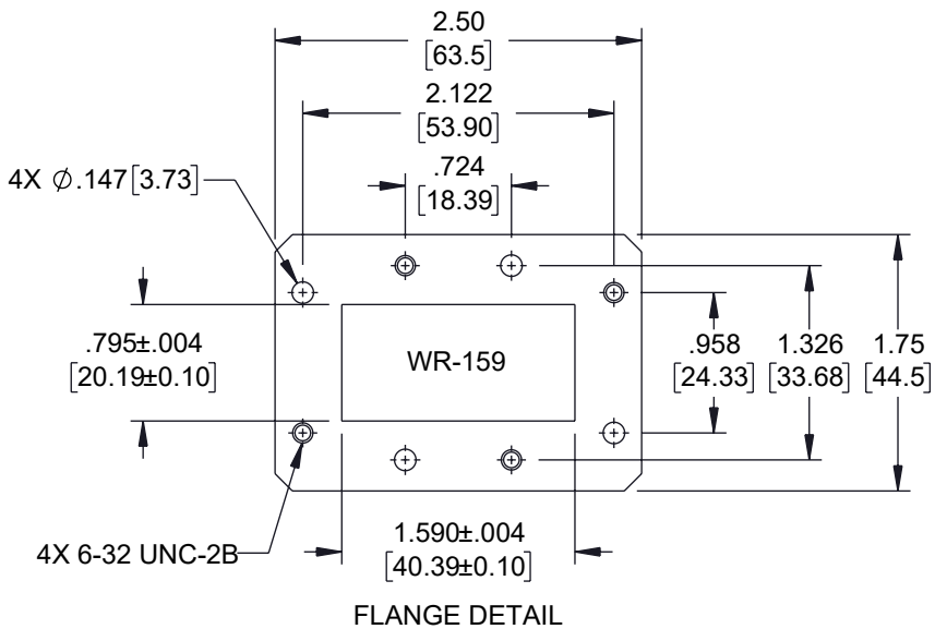
FLANGE DETAIL
