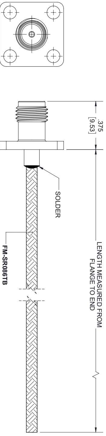
SMA FEMALE 4 HOLE FLANGE
