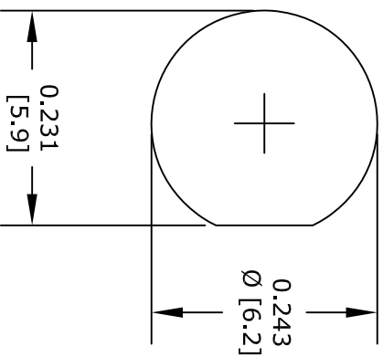
MOUNTING HOLE
