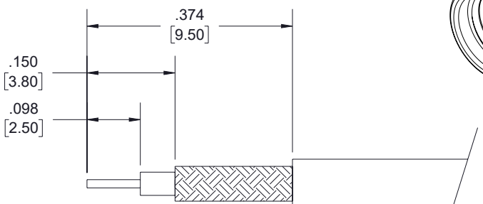
STRIPPING DIMENSIONS
