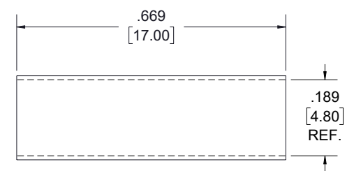
HEAT-SHRINK TUBING
