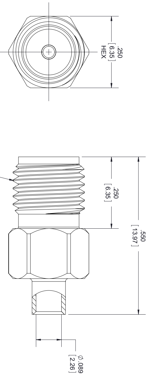
SMA FEMALE
