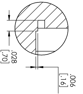
DETAIL B CENTER CONDUCTOR
