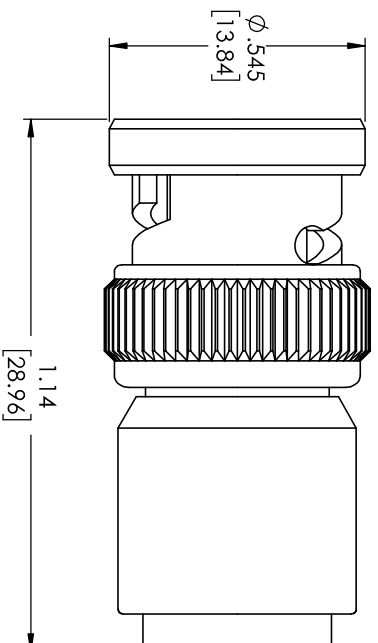
BNC MALE OPEN
