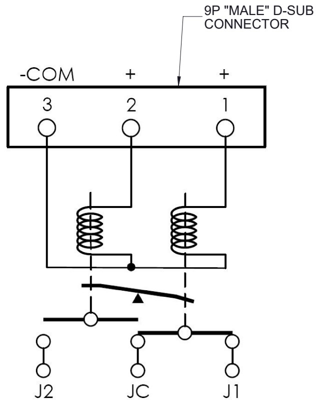
SCHEMATIC SHOWN IN LATCHING POSITION
