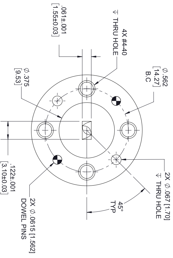
FLANGE DETAIL (BOTH SIDES)
