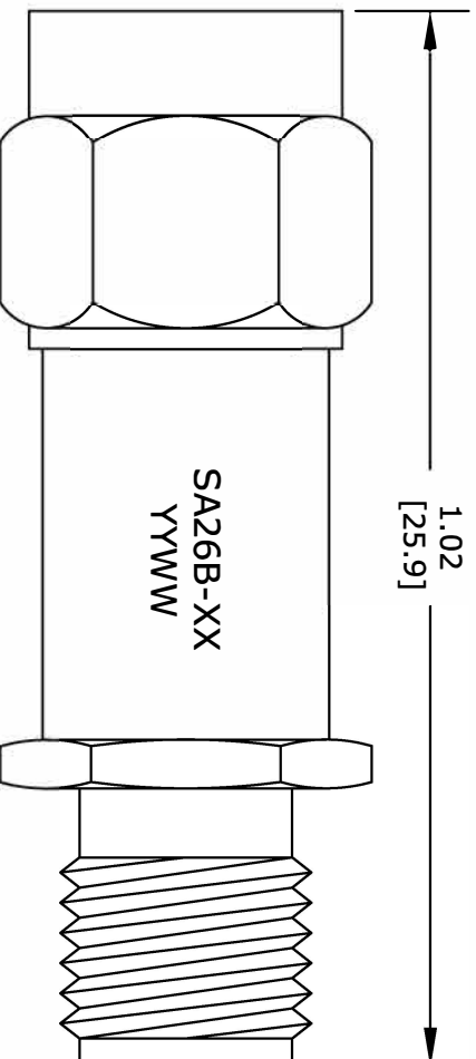
SMA MALE
