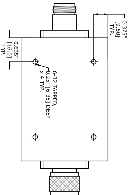
BOTTOM VIEW
