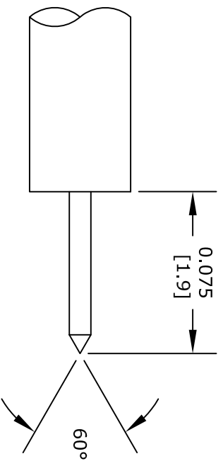
STRIPPING DIMENSIONS
