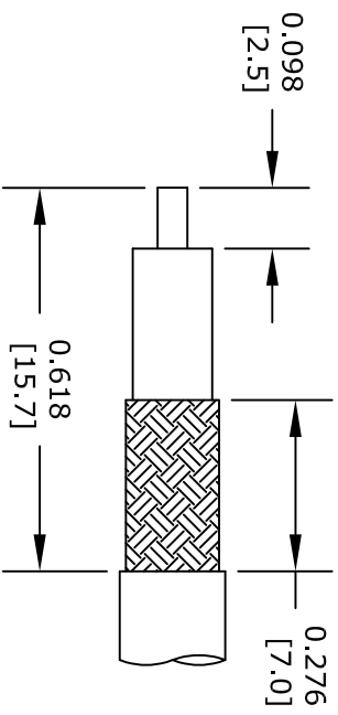
STRIPPING DIMENSION
