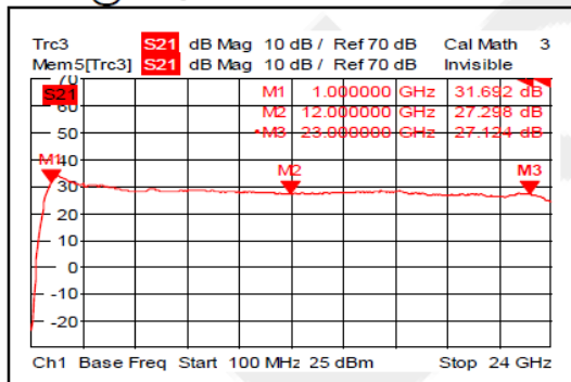
Gain @-45°C
