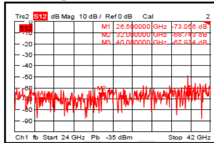
Isolation @-45°C
