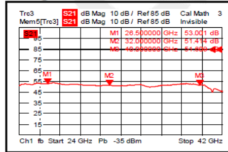
Gain @-45°C
