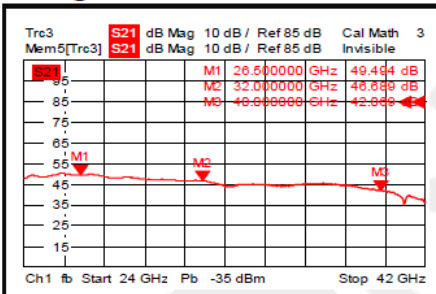
Gain @+85°C
