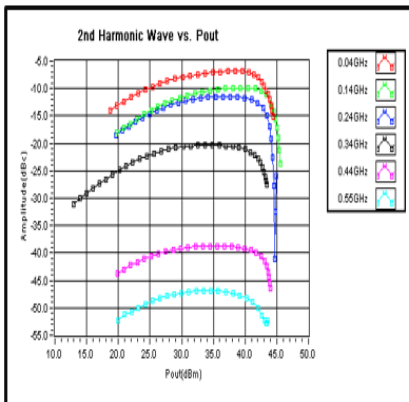
2nd Harmonic Wave Output Power
