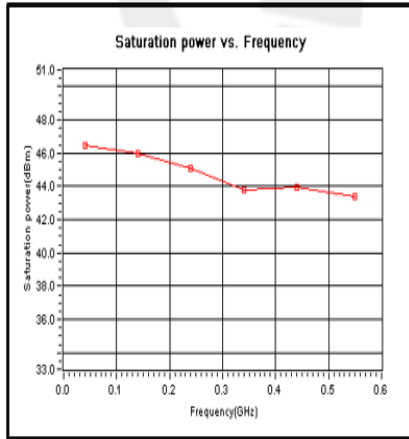
Saturated Power vs. Frequency
