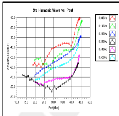
3rd Harmonic Wave Output Power
