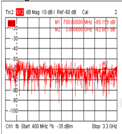
Isolation@+25°C
