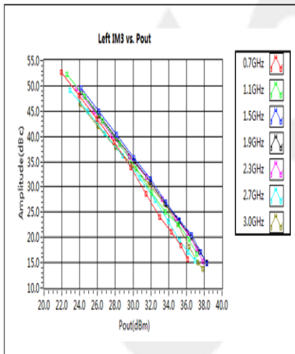
Left IM3 vs. Pout
