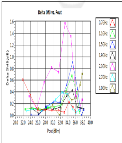
Delta IM3 vs. Pout
