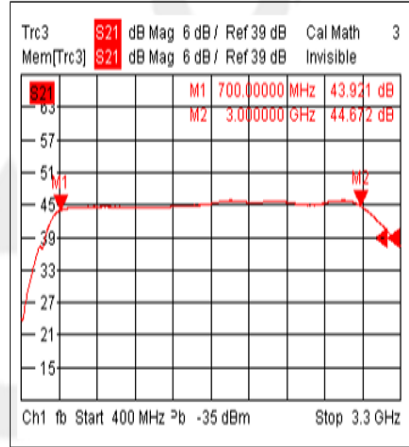
Gain@-40°C
