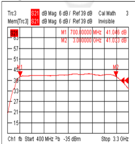
Gain@+70°C
