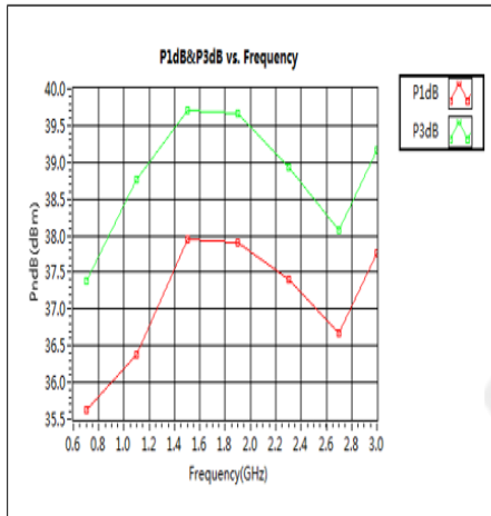
P1dB & P3dB vs. Frequency
