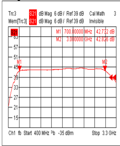
Gain@+25°C
