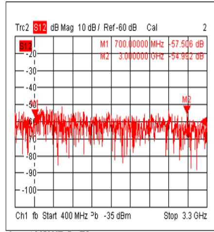
Isolation@-40°C
