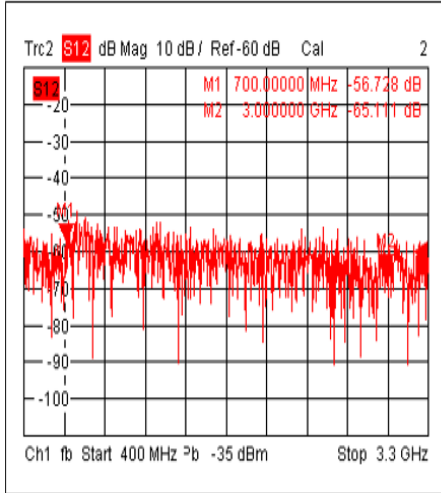
Isolation@+70°C
