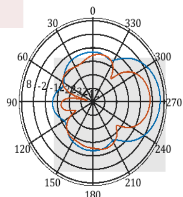
f=920MHz,X-Y Plane
