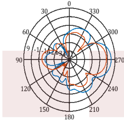
f=900MHz,@Y-Z plane
