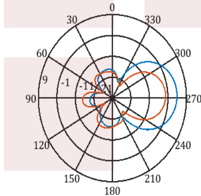
f=900MHz,X-Y Plane
