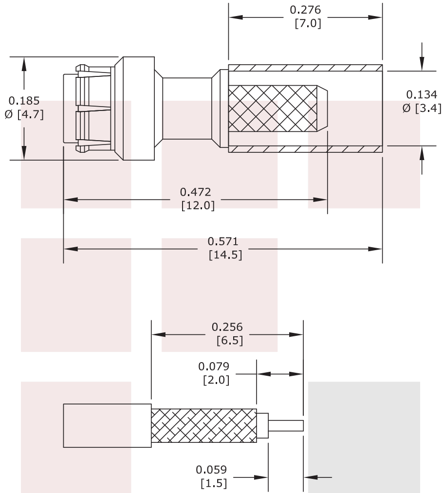
STRIPPING DIMENSIONS
