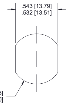
MOUNTING HOLE (2X)
