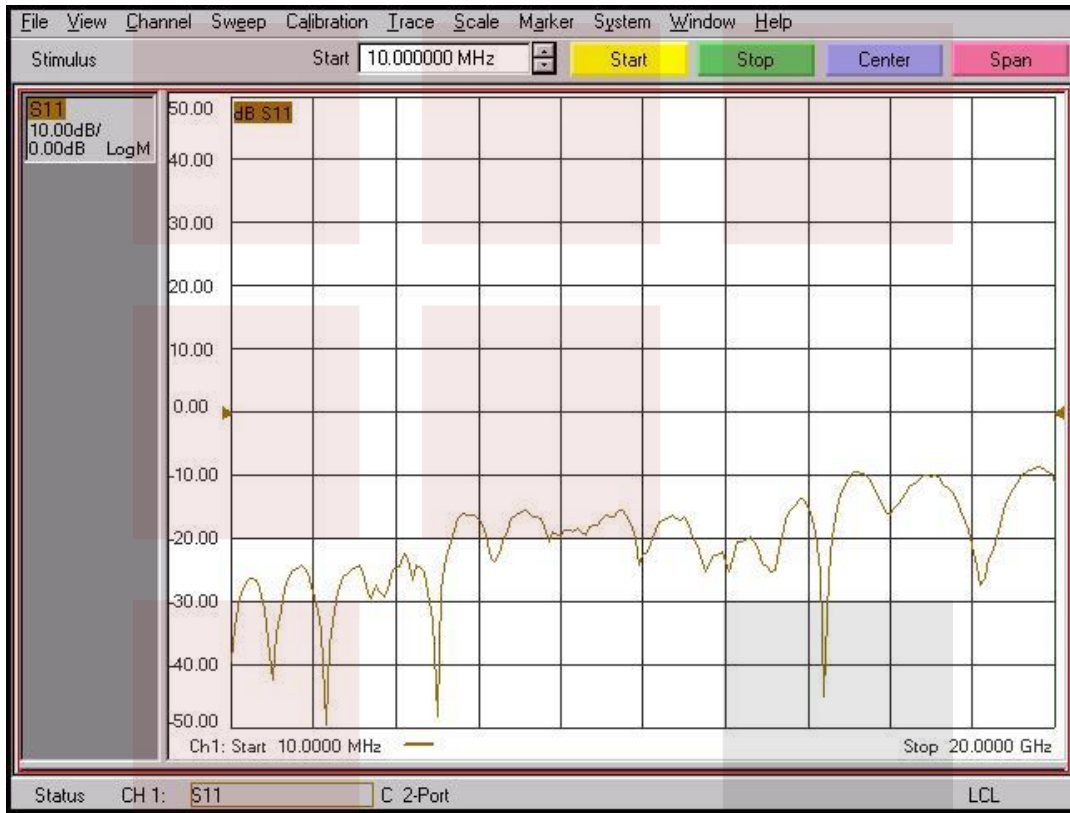
TEST DATA TAKEN WITH 2 FMPB1000 PROBES (IN/OUT) ON EITHER END OF A 40mm COPLANAR WAVEGUIDE
