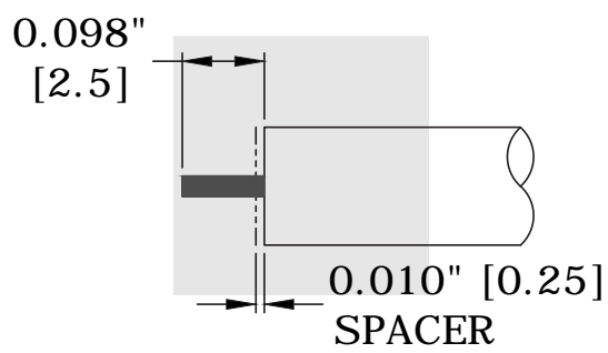
STRIPPING DIMENSION
