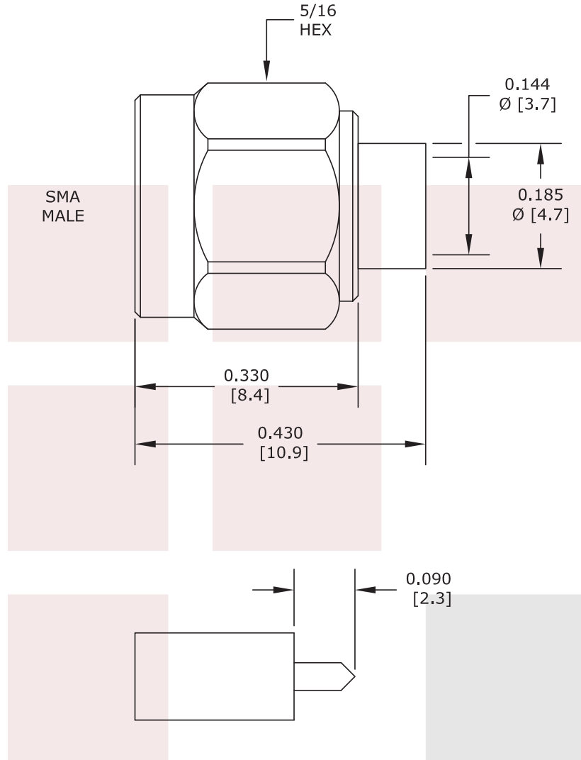
STRIPPING DIMENSIONS
