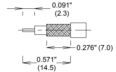
STRIPPING DIMENSIONS
