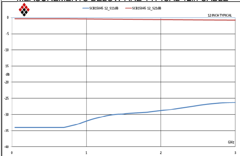
MEASUREMENTS BELOW ARE TYPICAL 12in CABLE
