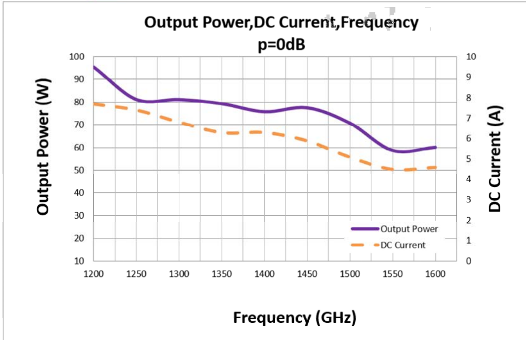
Graph3: Output Power(Normal temp.+25±3°C)
