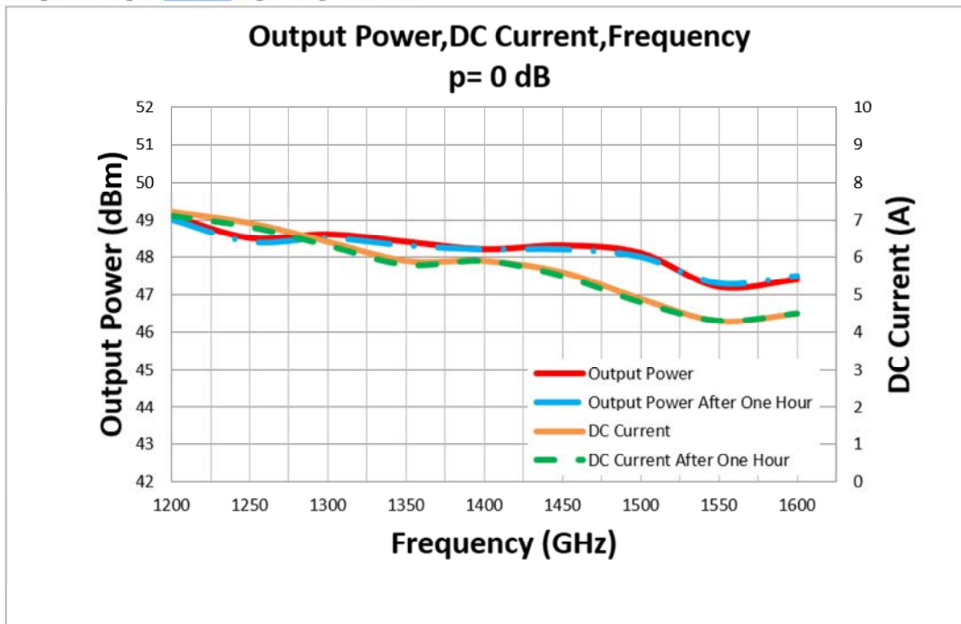
Graph2: Output Power(High temp.+80±3°C)
