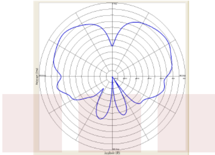
Figure 2: Radiation pattern on ground plane at 1575 MHz (RHCP)
