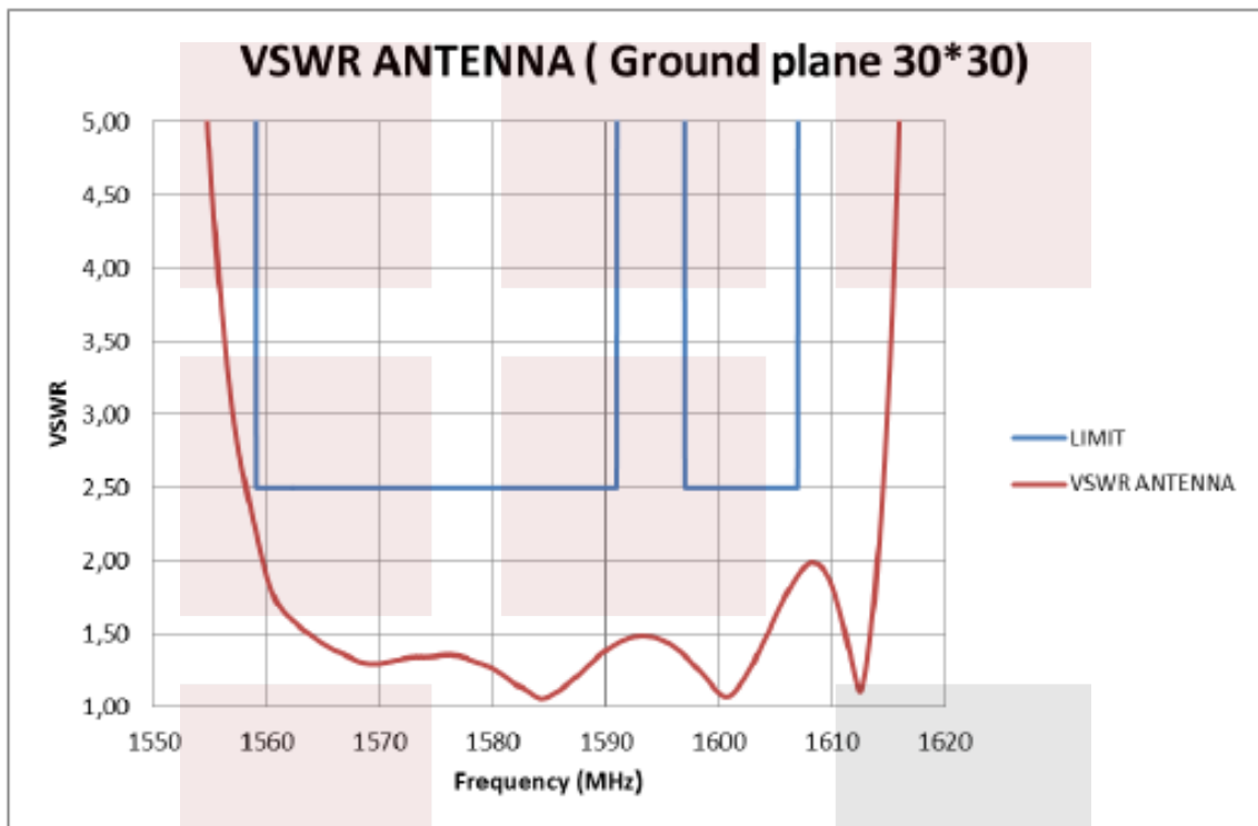
Figure 1: VSWR
