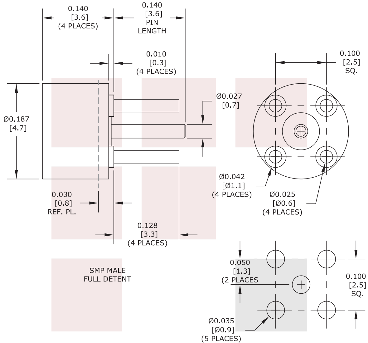
MOUNTING HOLES
