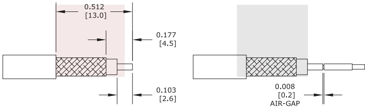
STRIPPING DIMENSIONS
